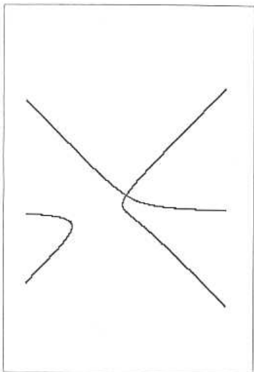
FIG. 1: A coarse and a fine covering for the curve x^3 - xy^2 + x^2 - xy - y^2 = 0 (see Example 3 in §4).
