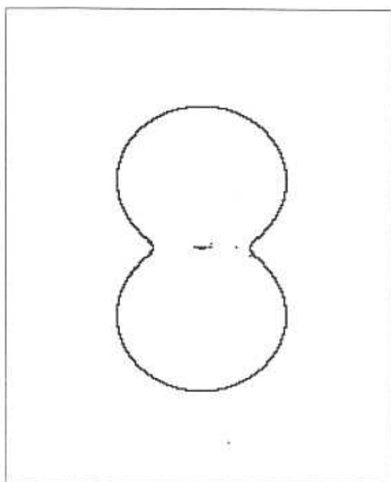
Fig. 3: A covering for the hippopede.
