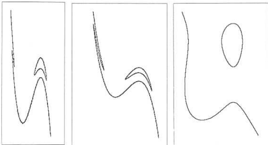
FIG. 2: (a) v_1 versus v_2 ; (b) v_1 versus v_2 ; (c) v_1 versus v_2 .
