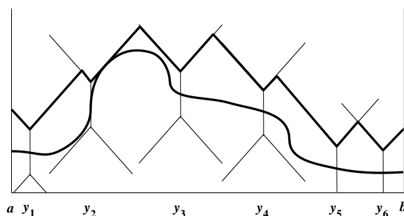
FIGURE 4. Continuous, non-Lipschitz, objective function and upper bounding function obtained from observations at y_1, y_2, \dots, y_6 .
